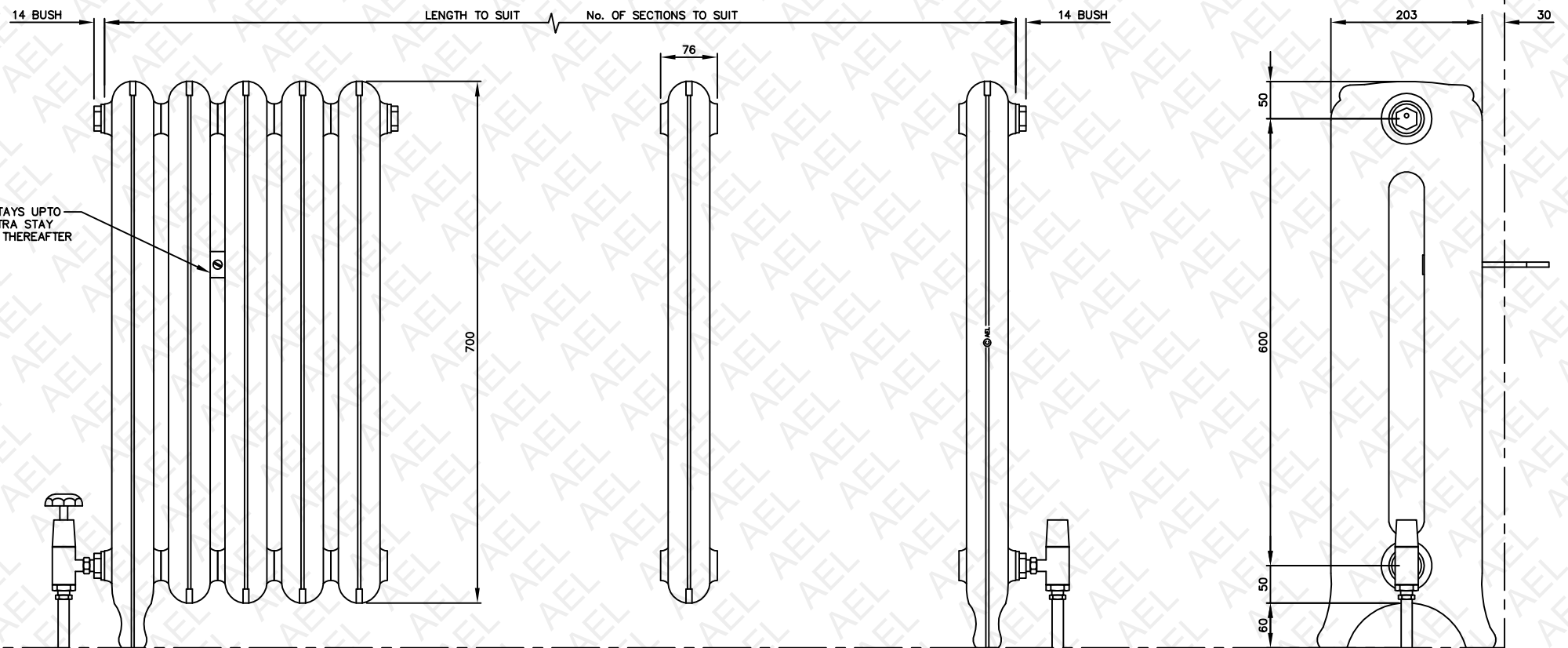
AEL HEATING SOLUTIONS ROYAL CAST IRON RADIATOR VR750
