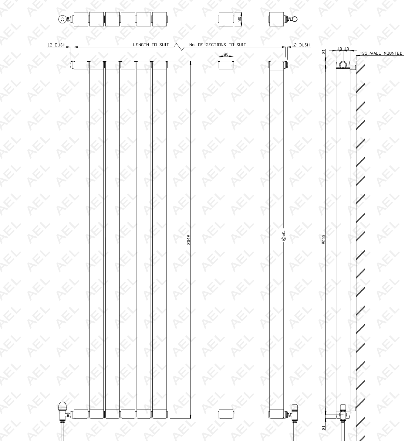
AEL HEATING SOLUTIONS VERTICAL LONGO ALUMINIUM RADIATOR VL80-2000
