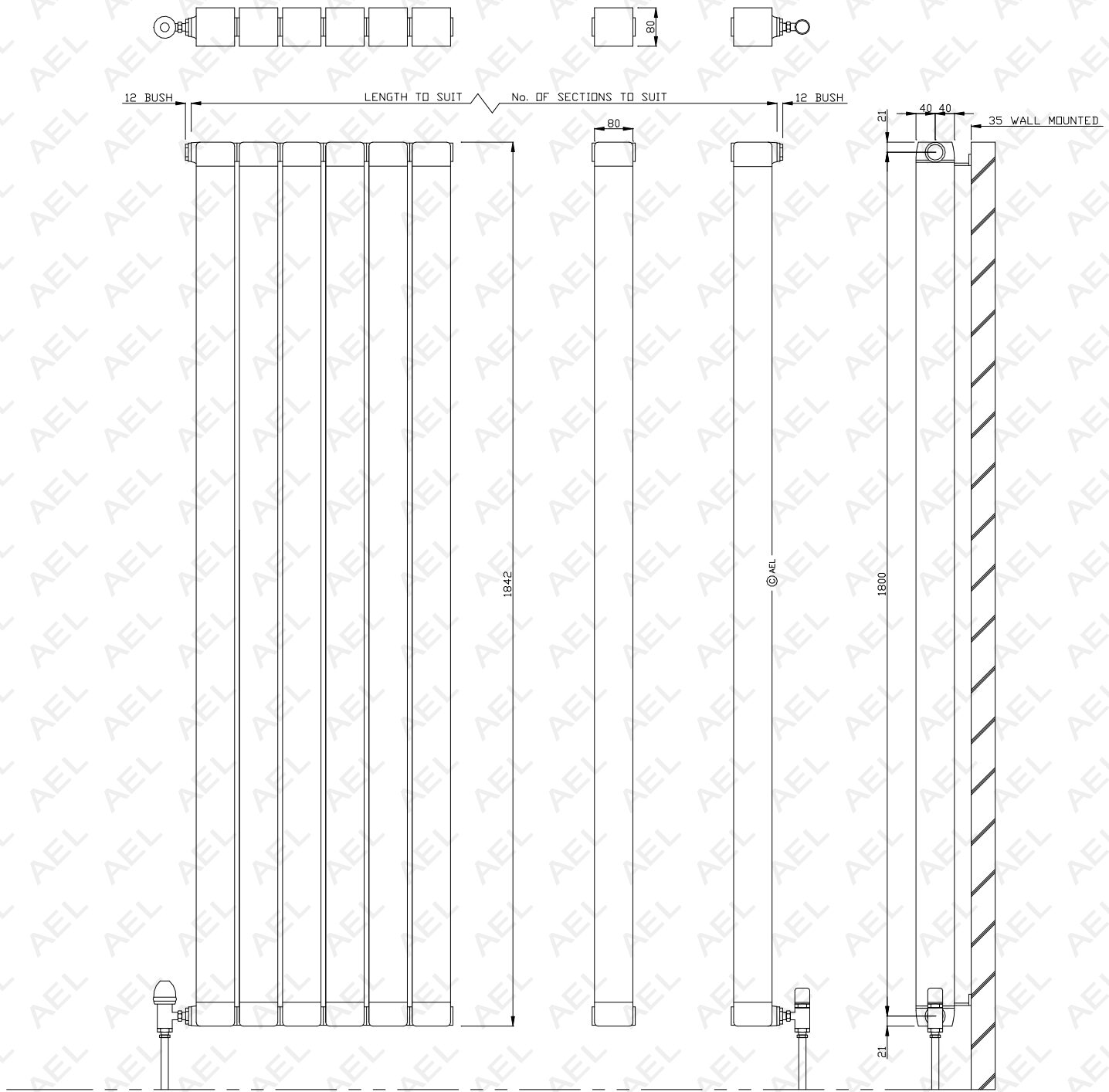
AEL HEATING SOLUTIONS VERTICAL LONGO ALUMINIUM RADIATOR VL80-1800
