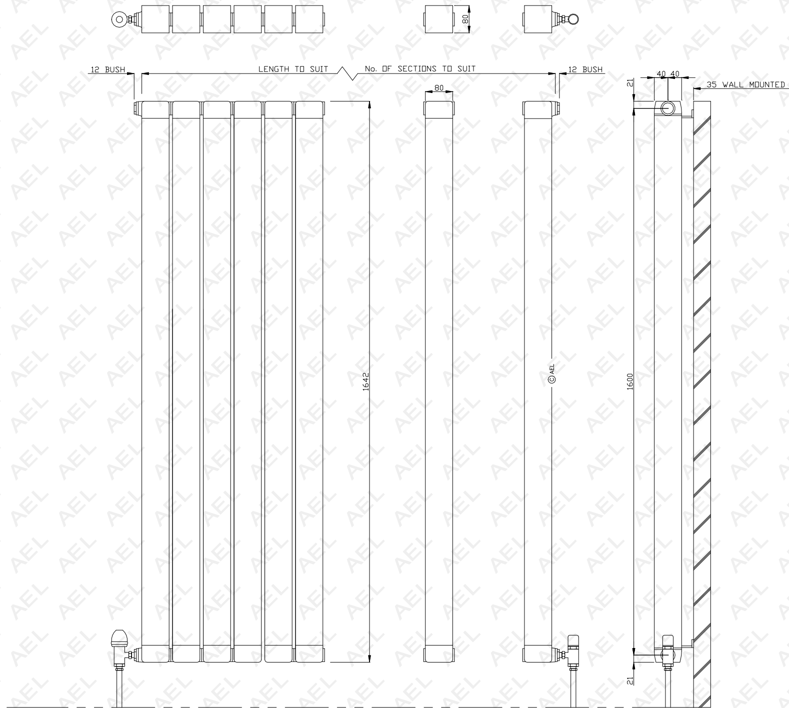
AEL HEATING SOLUTIONS VERTICAL LONGO ALUMINIUM RADIATOR VL80-1600
