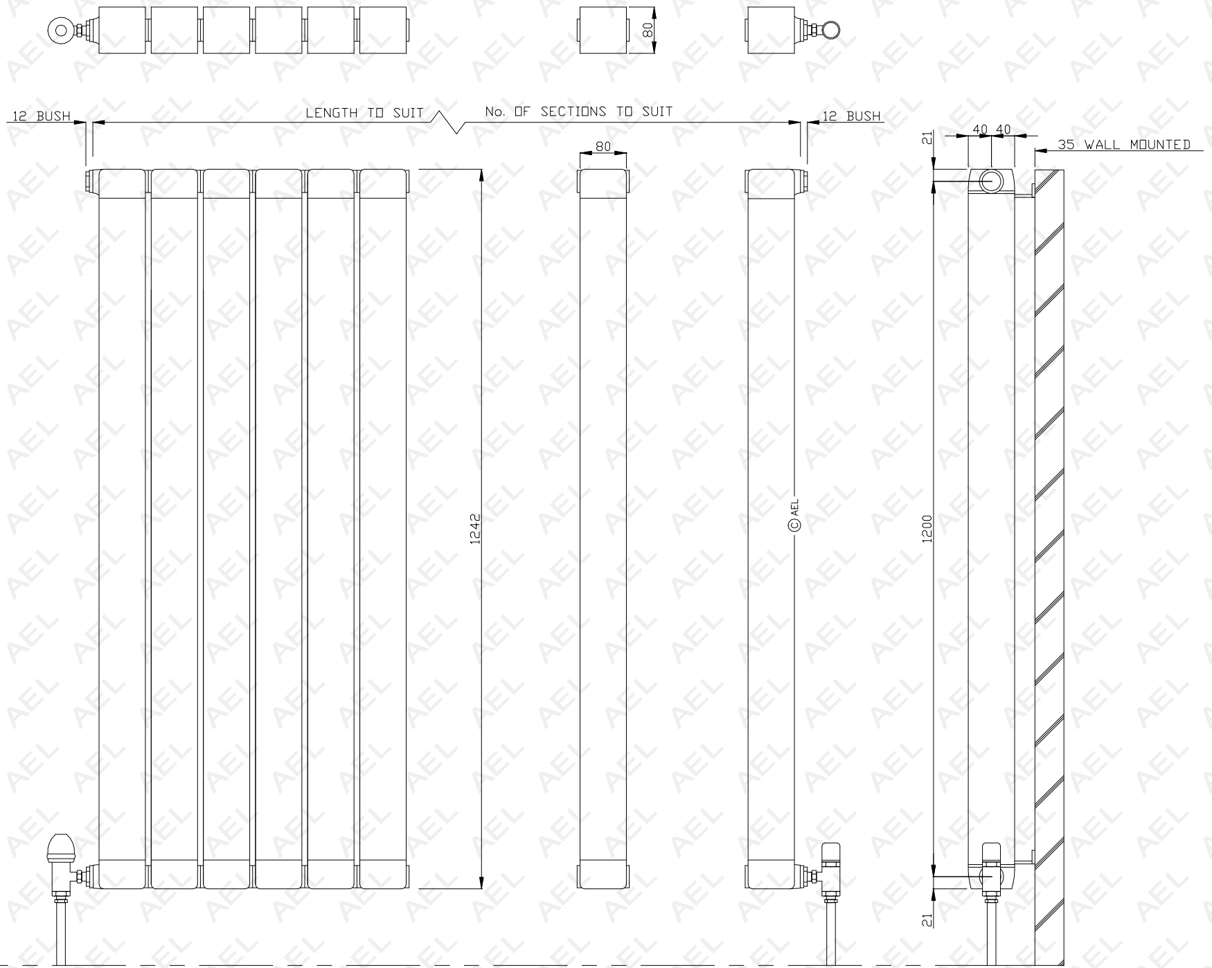
AEL HEATING SOLUTIONS VERTICAL LONGO ALUMINIUM RADIATOR VL80-1200
