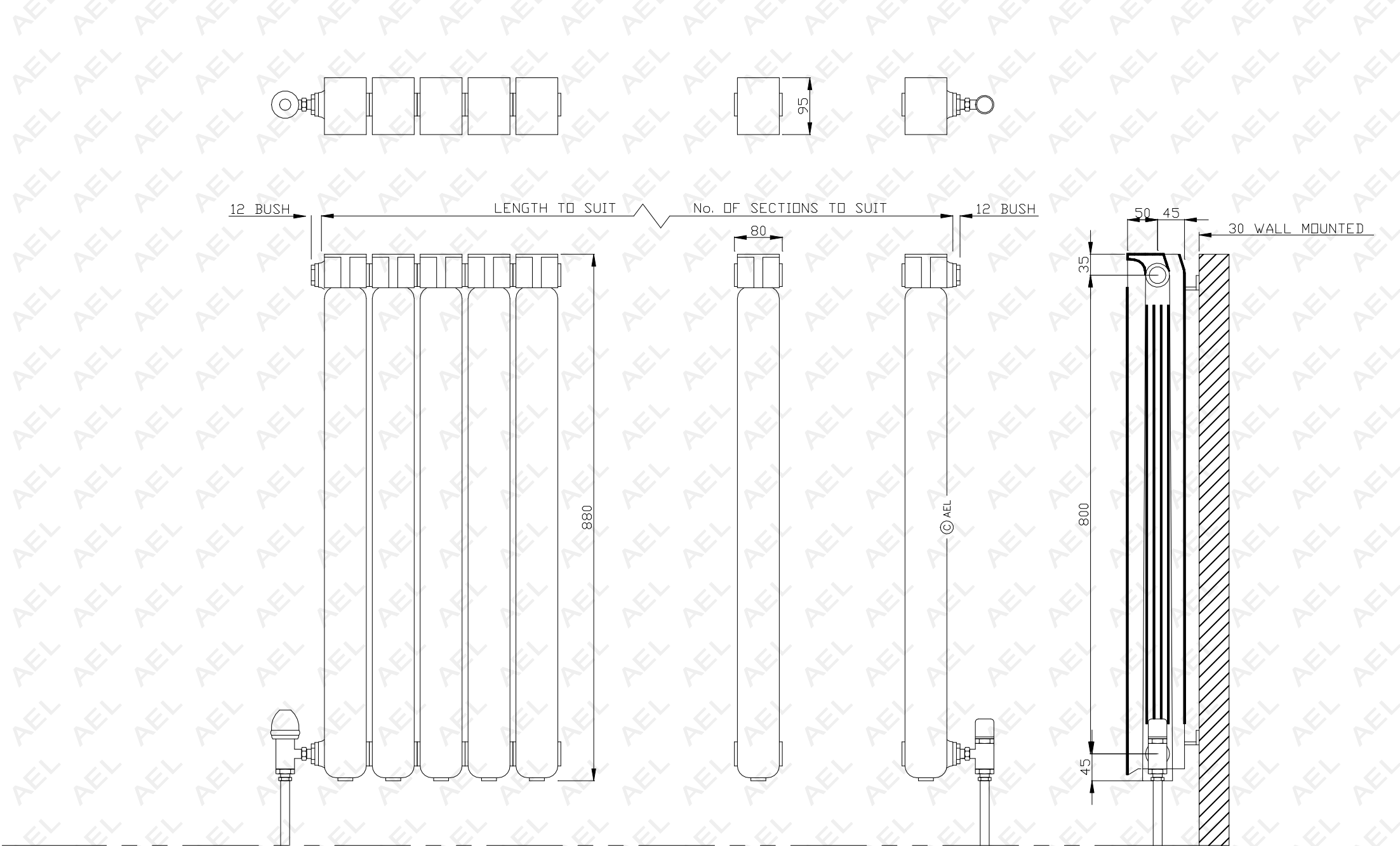
AEL HEATING SOLUTIONS FARAL TROPICAL 95 ALUMINIUM RADIATOR T95-880
