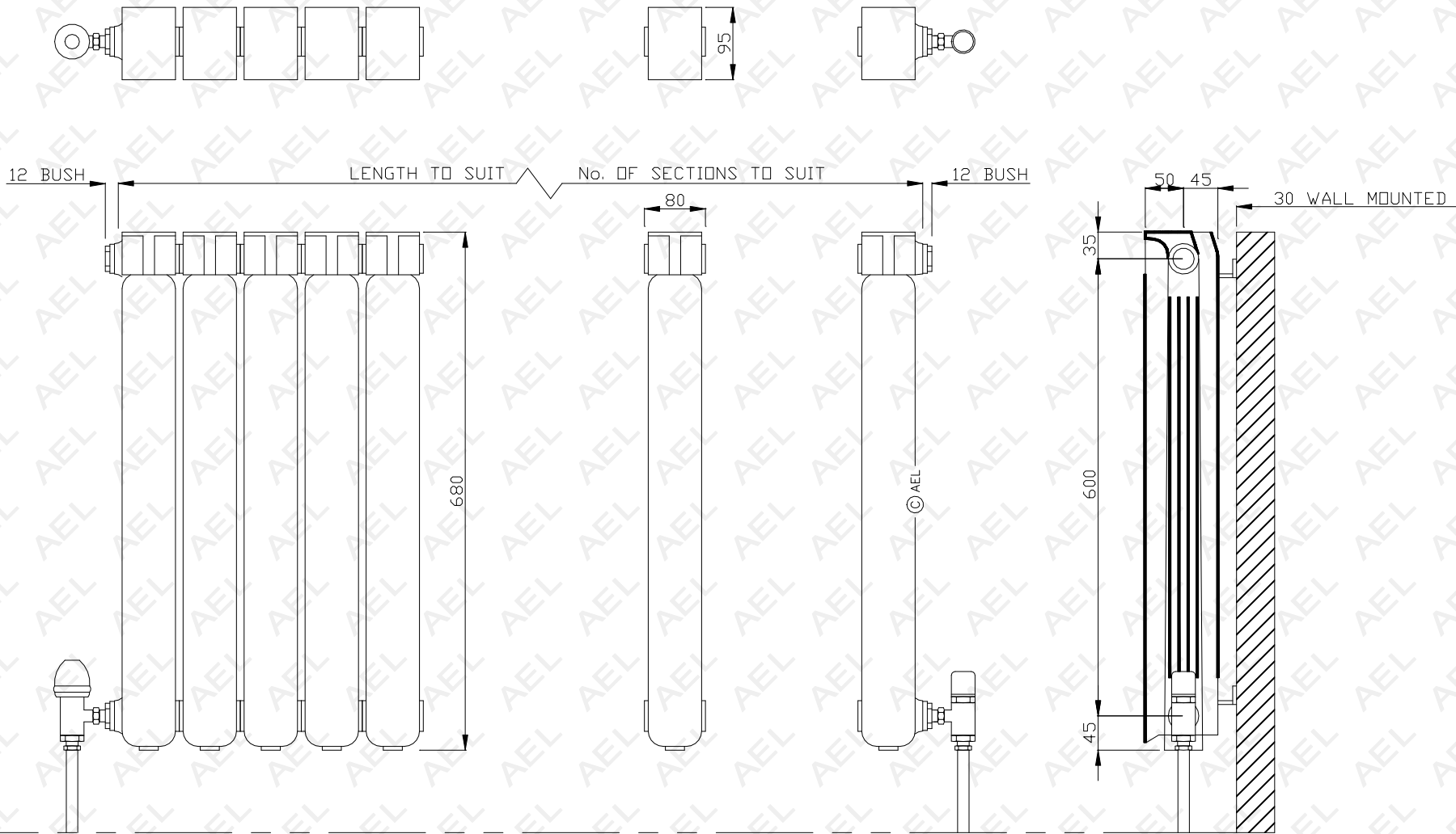
AEL HEATING SOLUTIONS FARAL TROPICAL 95 ALUMINIUM RADIATOR T95-680
