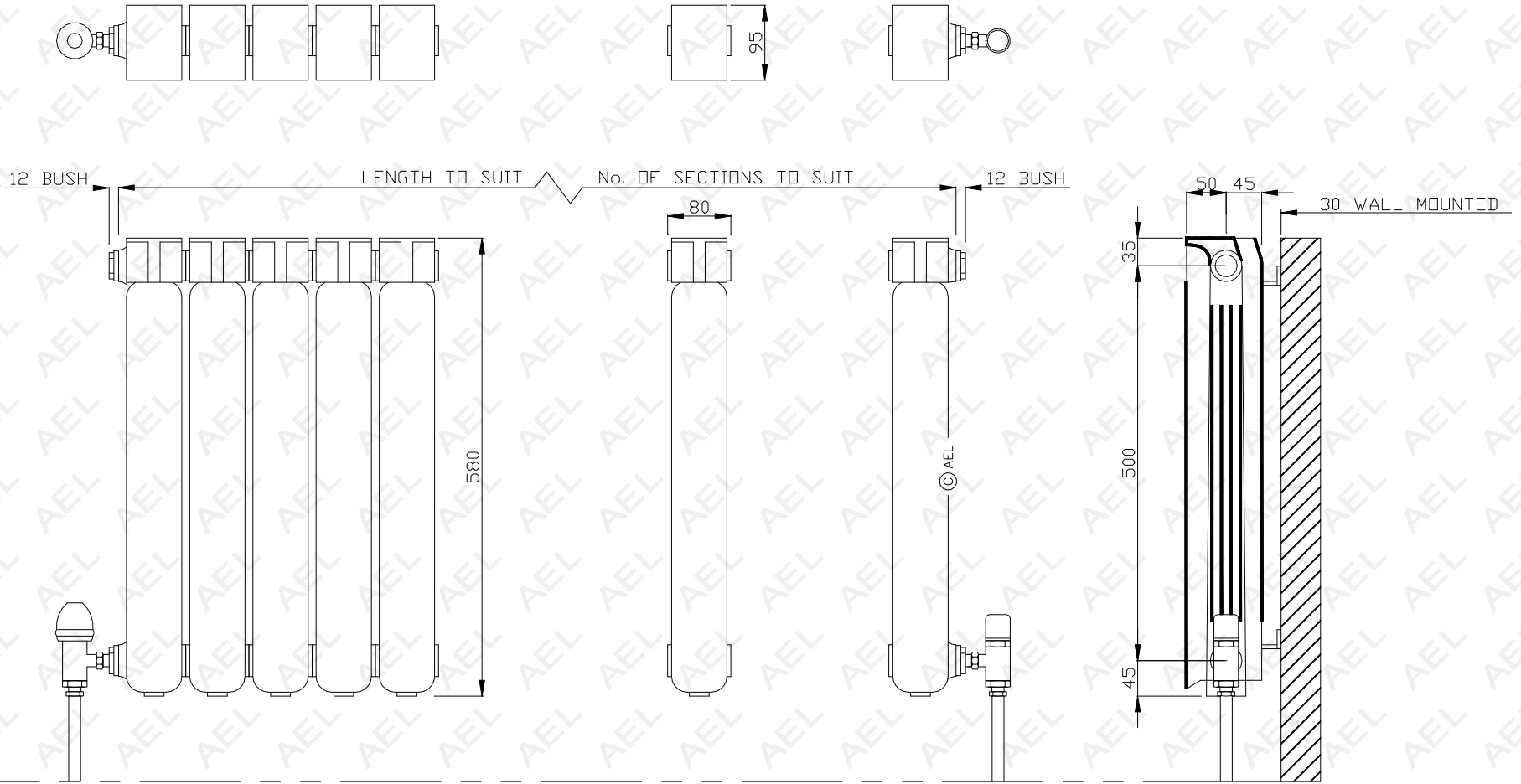
AEL HEATING SOLUTIONS FARAL TROPICAL 95 ALUMINIUM RADIATOR T95-580
