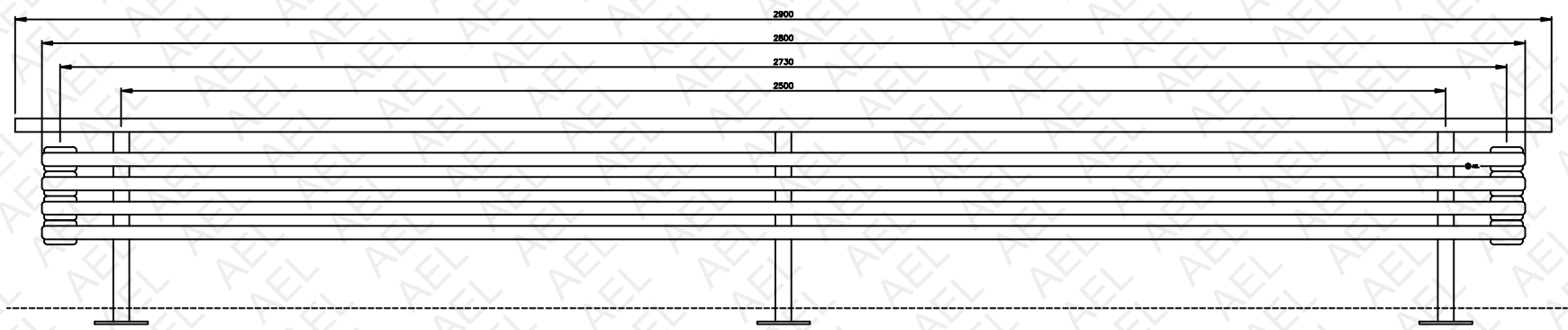
AEL HEATING SOLUTIONS BENCHRAD BENCH TYPE RADIATOR F8280/4
