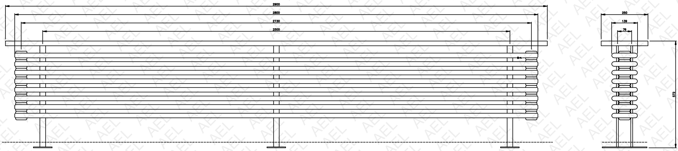
AEL HEATING SOLUTIONS BENCHRAD BENCH TYPE RADIATOR P4280/8
