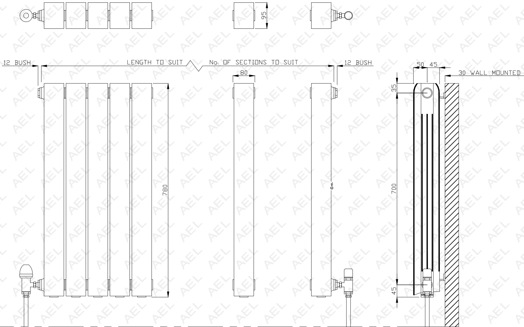
AEL HEATING SOLUTIONS FARAL ALLIANCE 95 ALUMINIUM RADIATOR FA95-780
