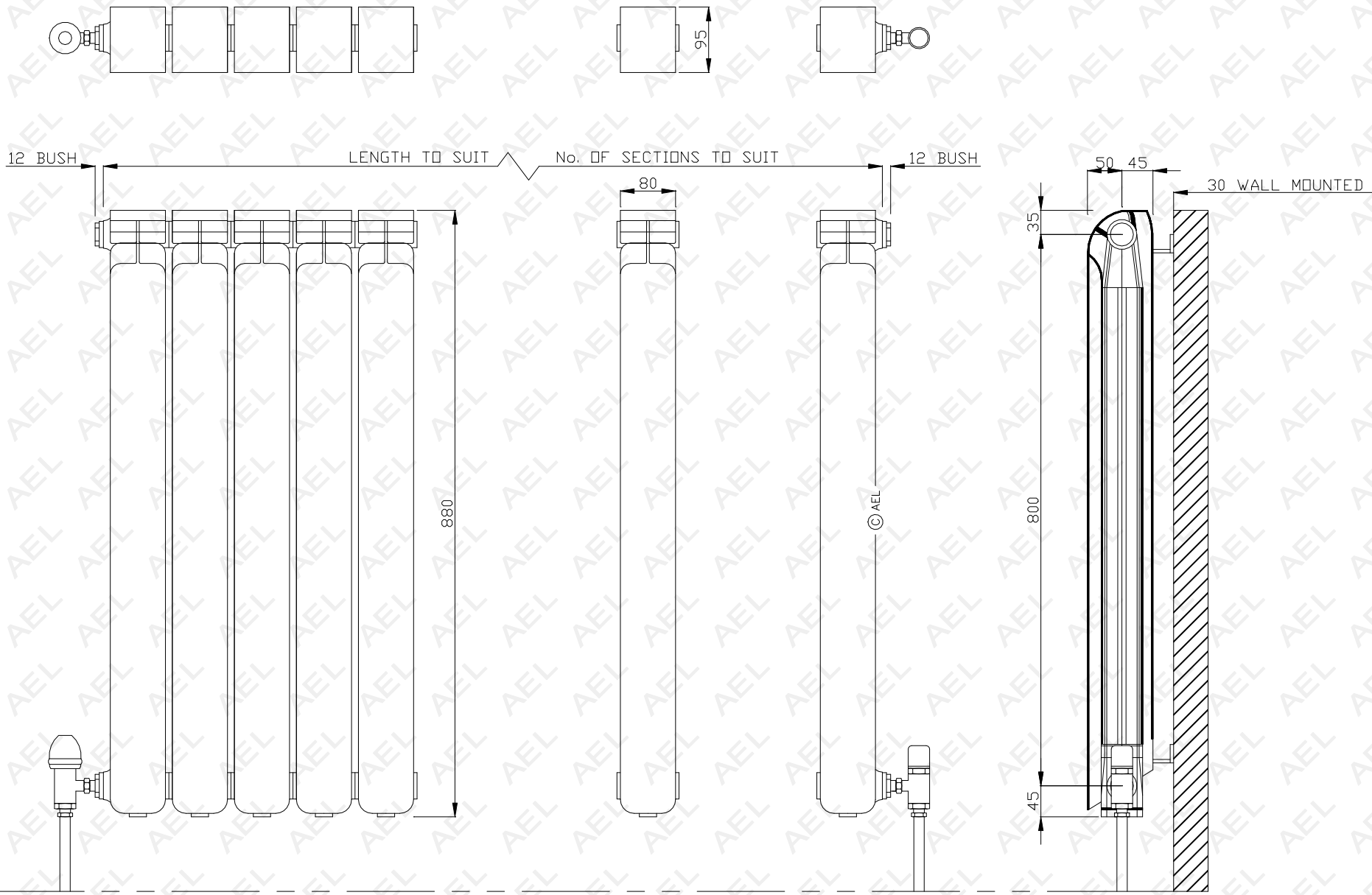
AEL HEATING SOLUTIONS FARAL ALBA 95 ALUMINIUM RADIATOR ALBA 95-880
