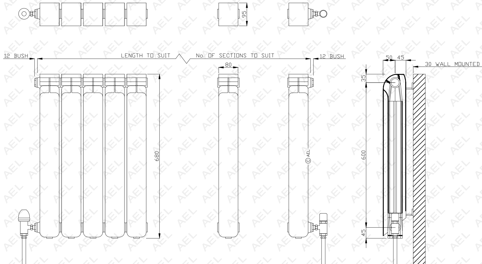
AEL HEATING SOLUTIONS FARAL ALBA 95 ALUMINIUM RADIATOR ALBA 95-680
